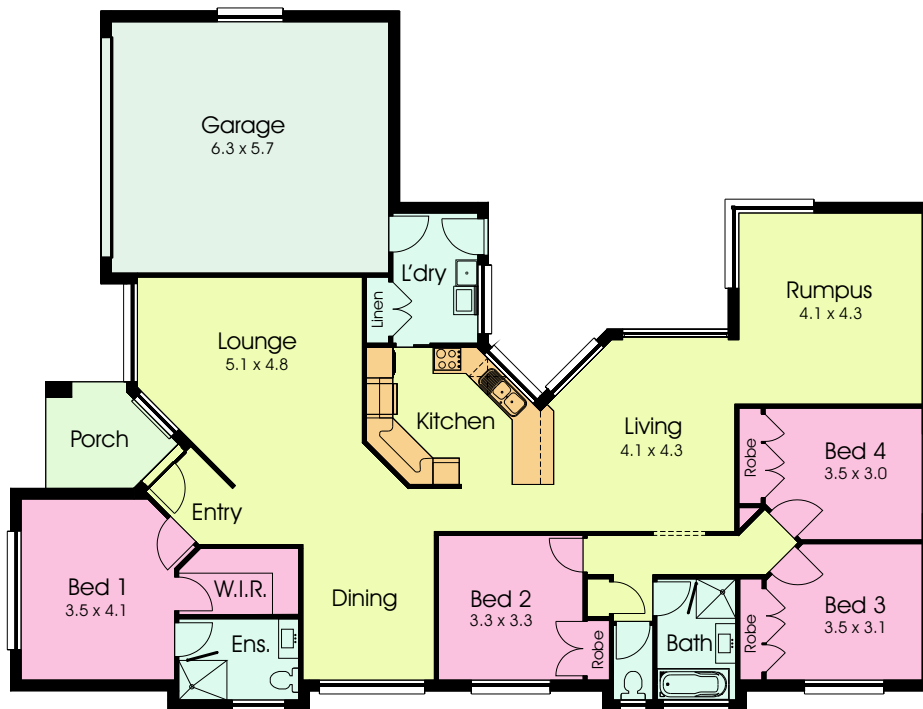
Floor Plan
